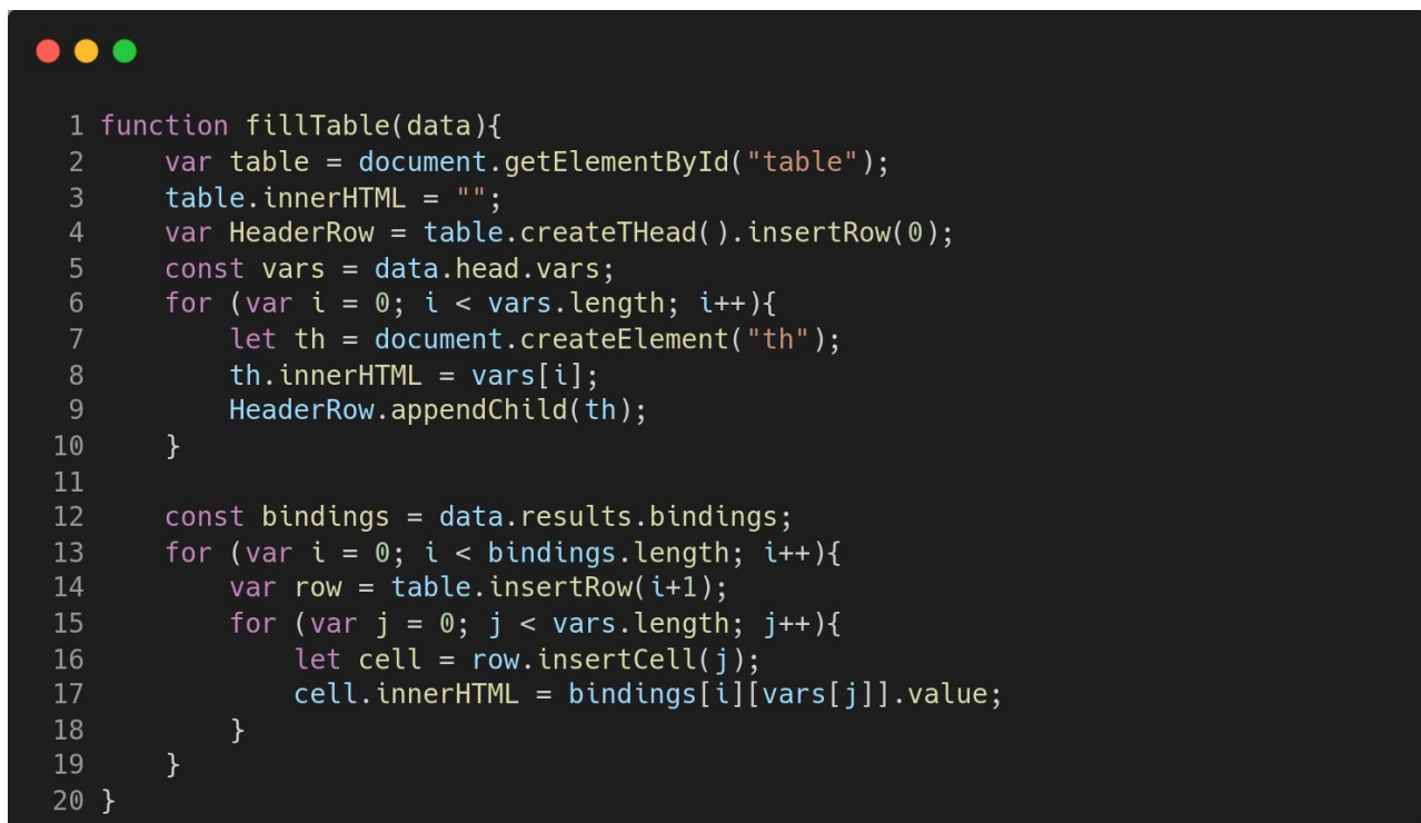
Implementation for generating a table from JSON data
